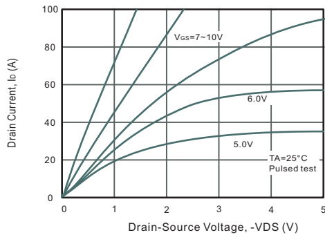
Fig.1 Output Characteristics
